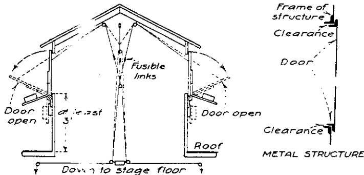
SECTION OF WOODEN VENTILATOR
