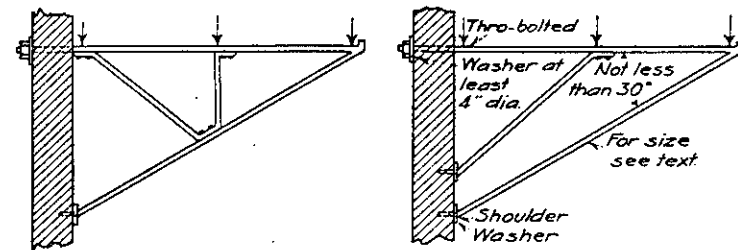
TWO TYPES OF TWO STAIR SUPPORT
