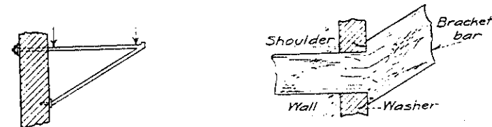
ONE STAIR SUPPORT DETAIL OF WALL BEARING TYPICAL FIRE ESCAPE BRACKETS
