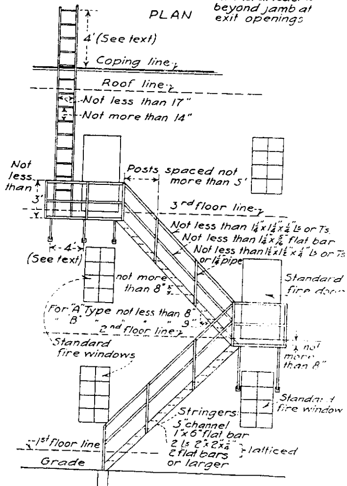
ELEVATION FIRE ESCAPES
