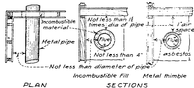
PLAN SECTIONS
