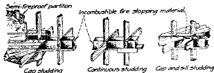
FIRE STOPPING
