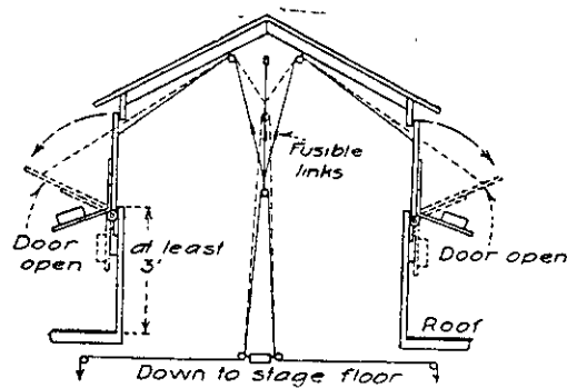
SECTION OF WOODEN VENTILATOR
