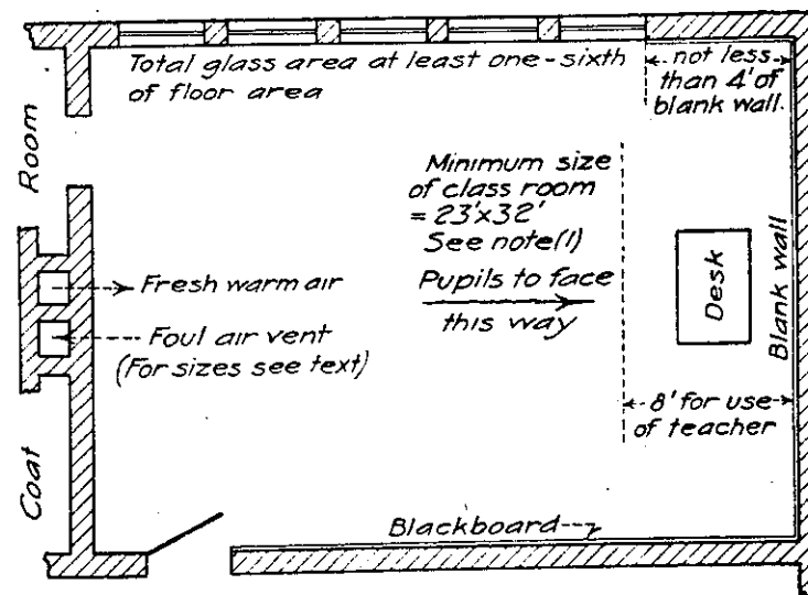
TYPICAL CLASS ROOM
