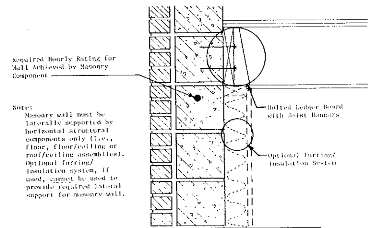
FIGURE 3 Multi-Wythe Masonry Wall (Bearing Condition)
