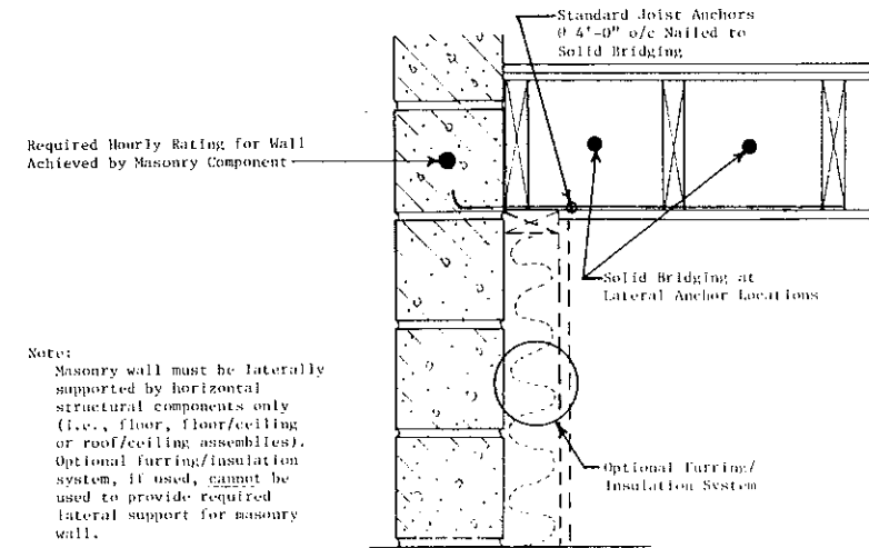
FIGURE 2 Single Wythe Masonry Wall (Non-Bearing Condition)
