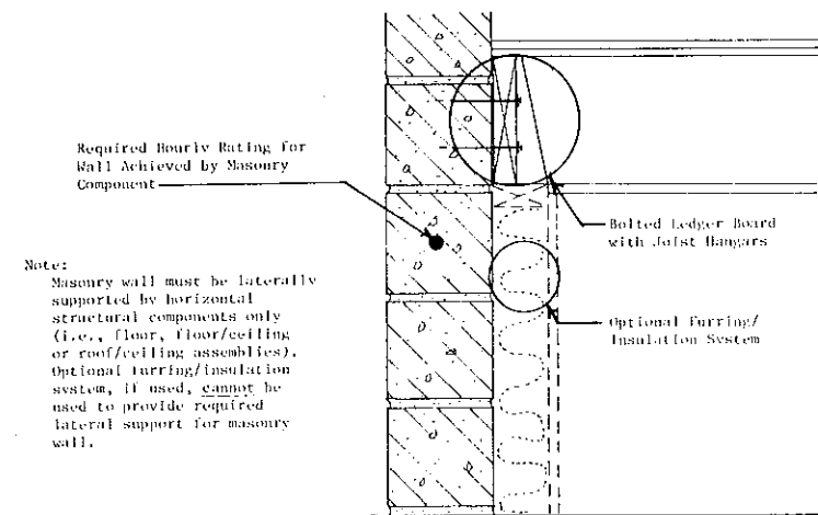
FIGURE 1 Single Wythe Masonry Wall (Bearing Condition)
