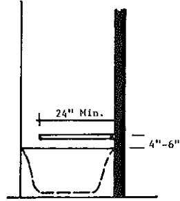
End Elevation - Bathtub
