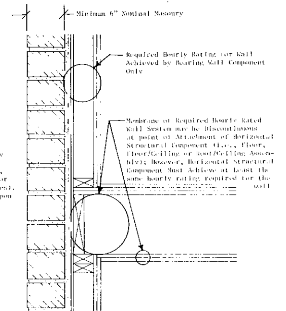
FIGURE 5B Combination Masonry/Frame Wall (Bearing and Non-Bearing Condition)
