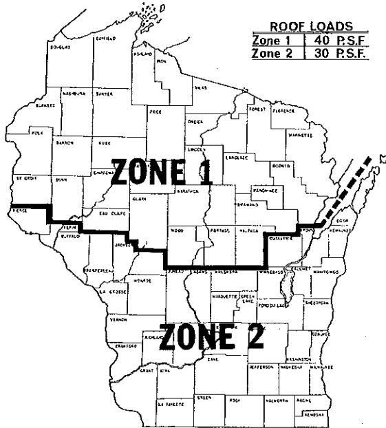
Zone Map for Roof Loads
